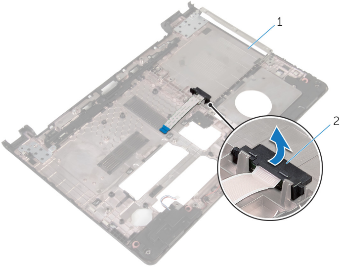
1 optical-drive interposer
